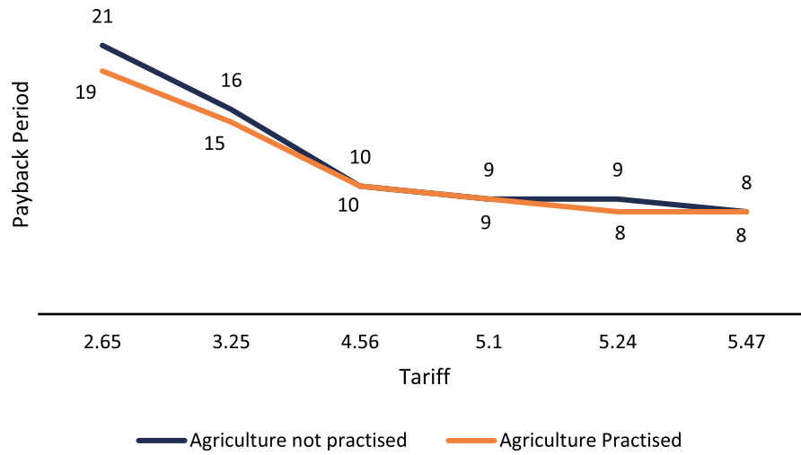
Figure C2: Payback Period of APV system at 6 m mounting height
